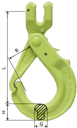
GBK SELF LOCKING HOOK
